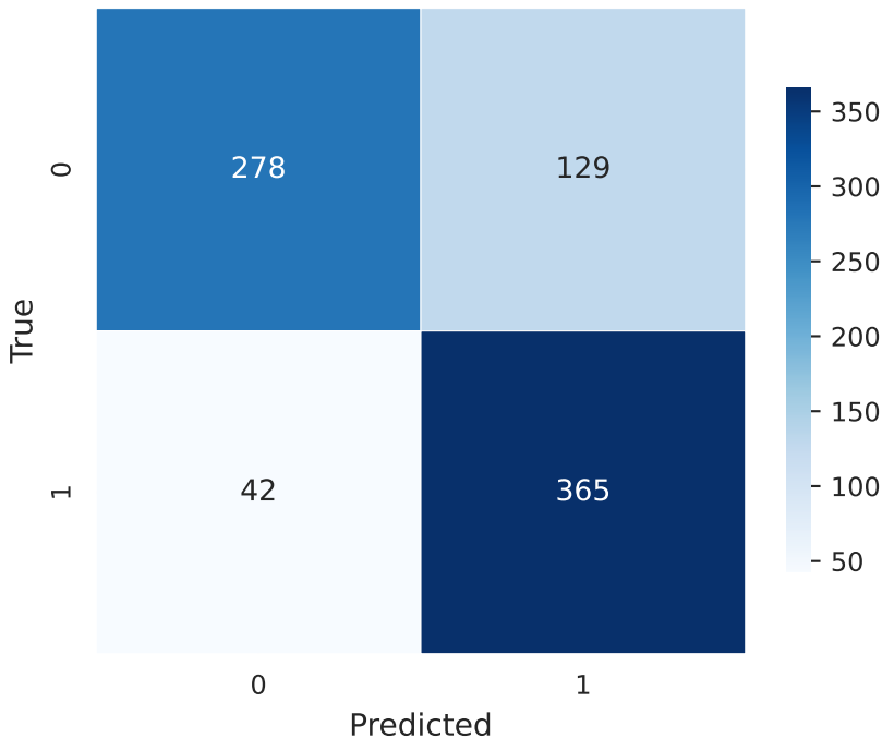
Confusion Matrix - sentence-biobert
