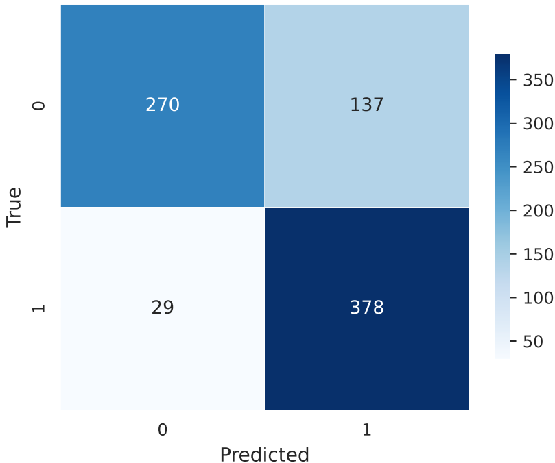
Confusion Matrix - e5-large
