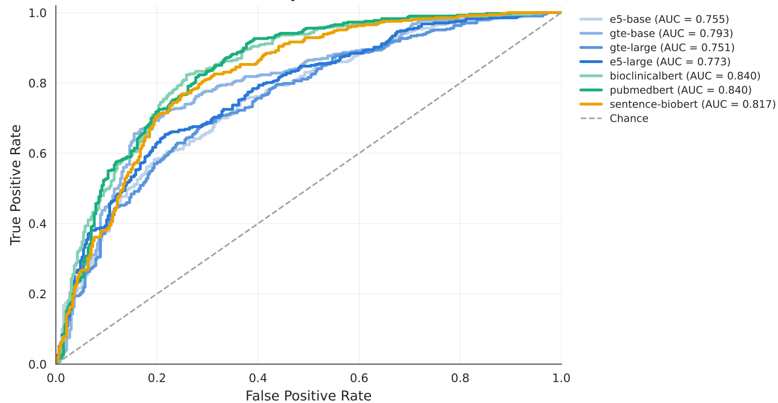
ROC Curve Comparison - All Models
