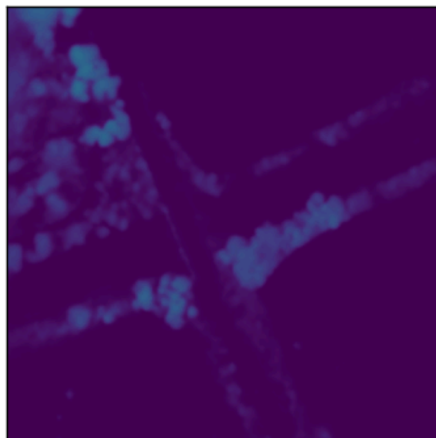
MSE Prediction
