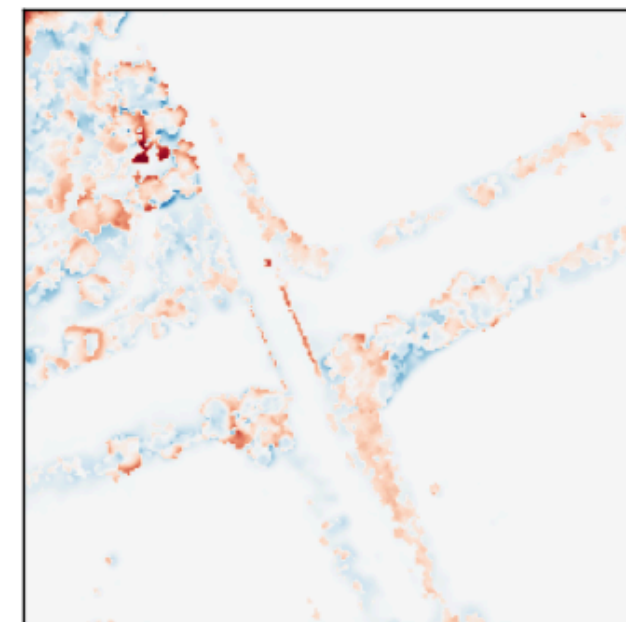
Residual Error
