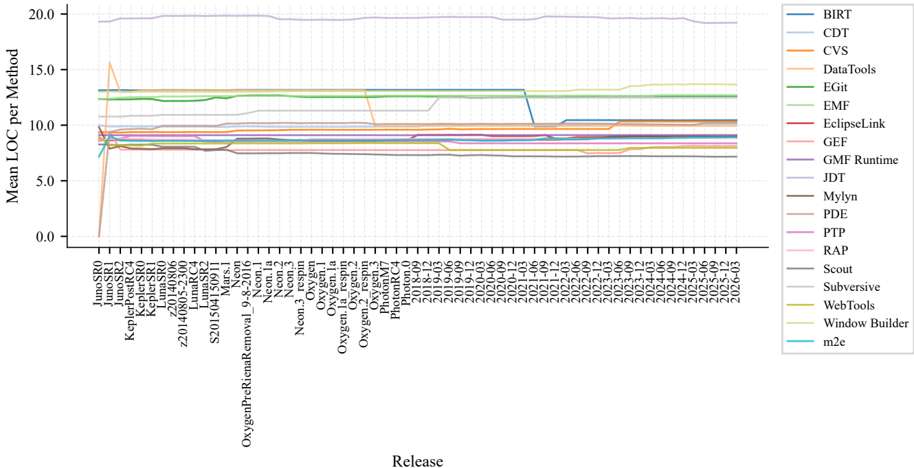
Mean LOC per Method per Feature Over Releases (All Features)
