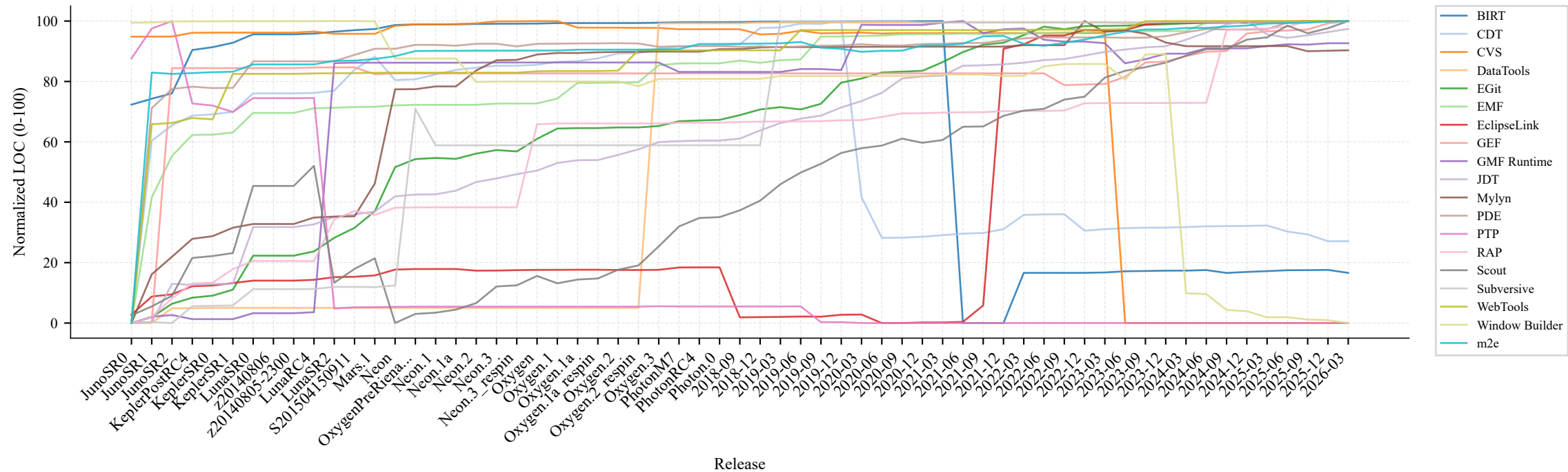
Normalized LOC per Feature Over Releases (All Features)
