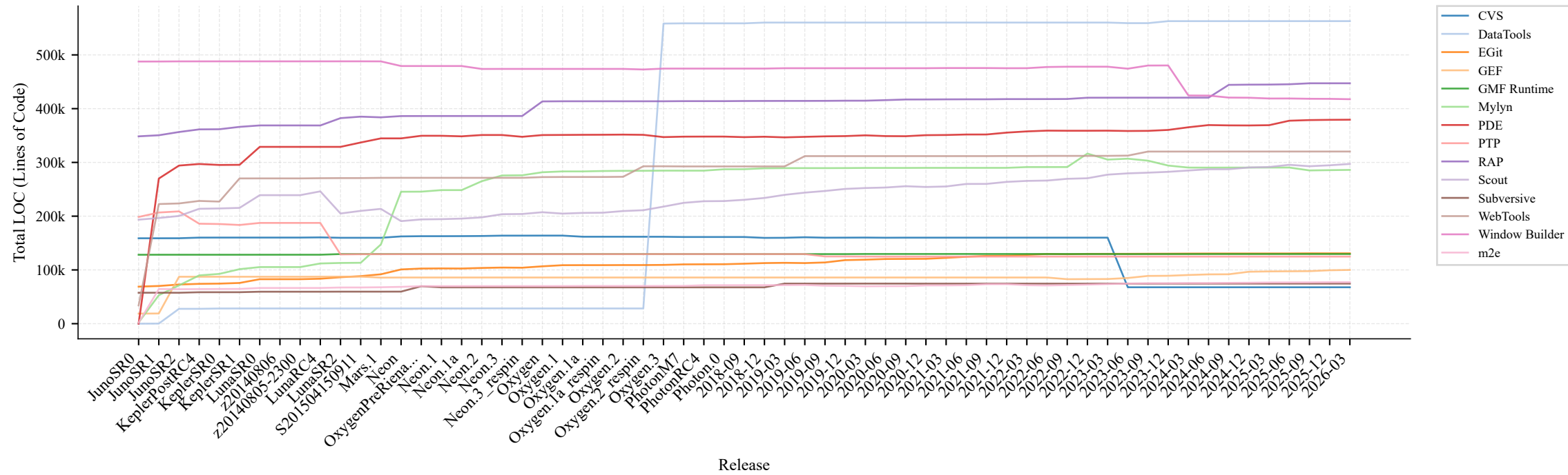
Total LOC per Feature Over Releases (Small Features)
