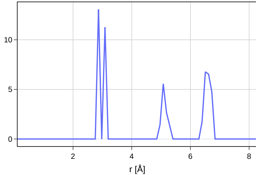
RDF Analysis
