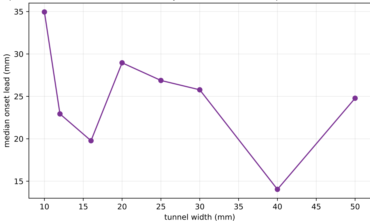
p09: median canonical onset lead by width (263 of 562 kept events drift-corrected)
