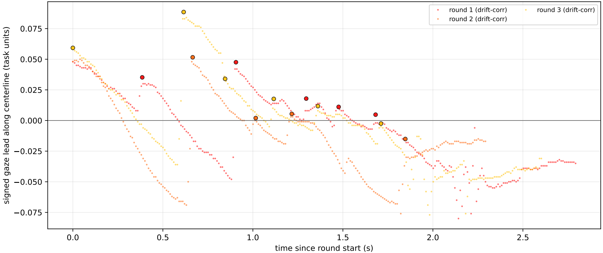
t57 constrained_to_unconstrained W=10mm (3/3 rounds drift-corrected; black-edged = canonical fixation onsets; ABC-style glob
