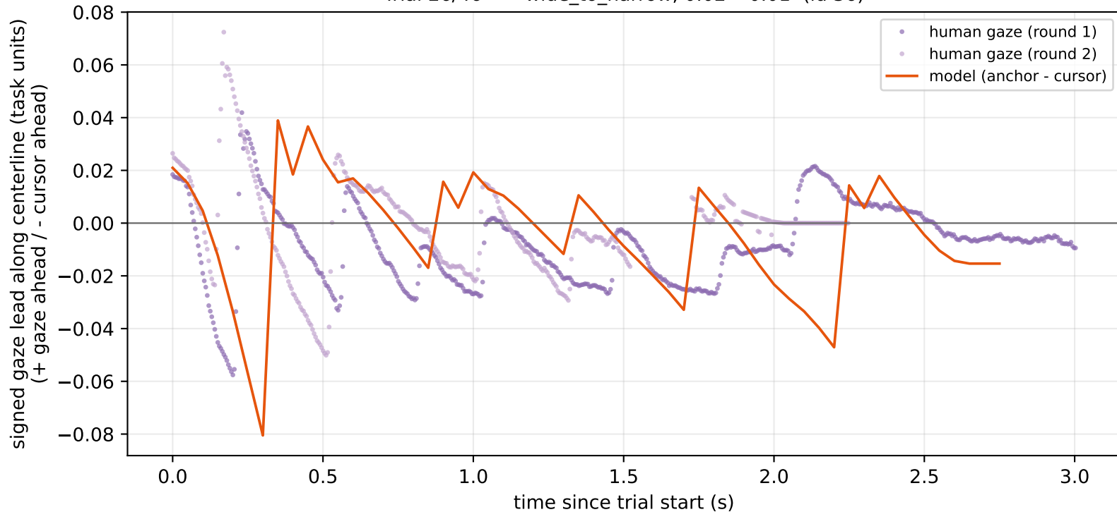
Trial 26/46 — wide_to_narrow, 0.02->0.01 (id 36)
