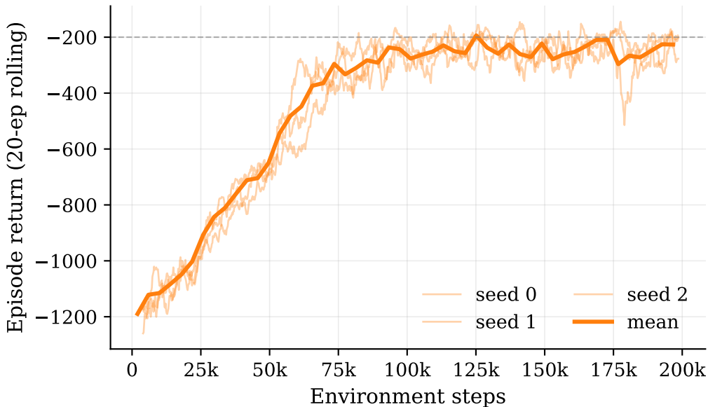
PPO on Pendulum-v1: per-seed curves
