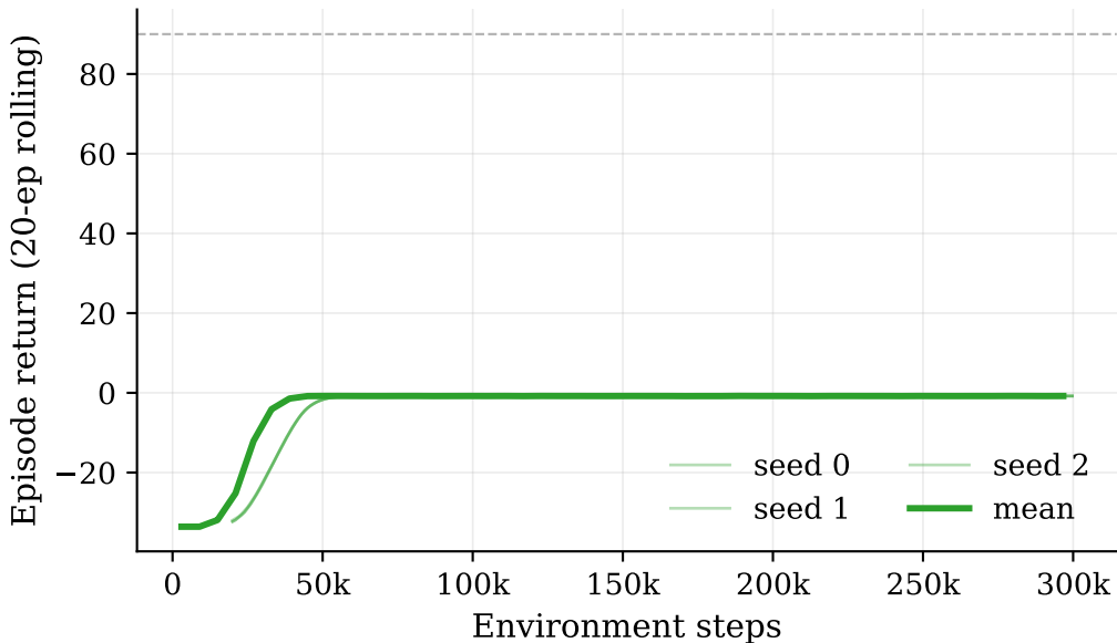
SAC on MountainCarContinuous-v0: per-seed curves
