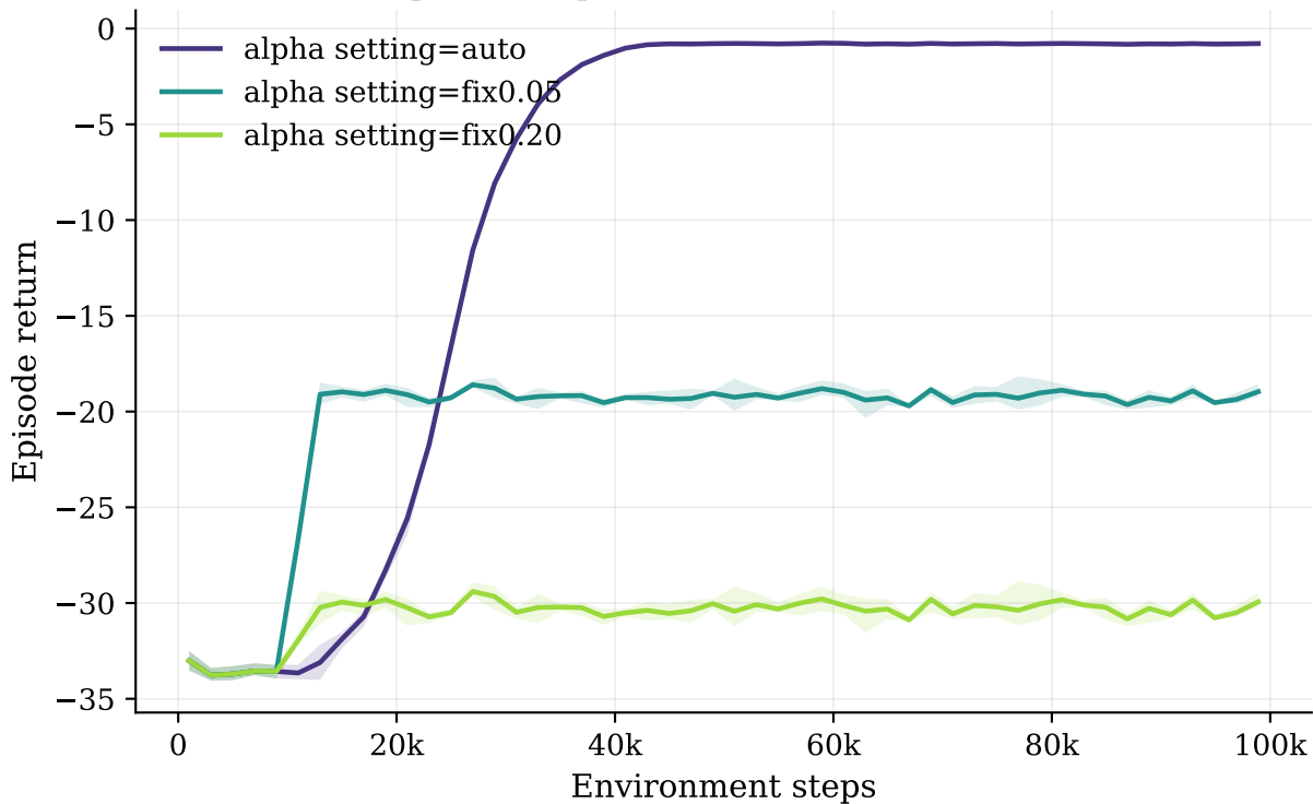
SAC alpha sweep on MountainCarContinuous-v0
