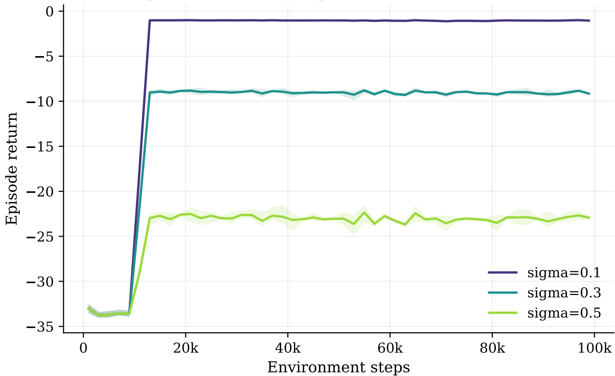
TD3 exploration noise sweep on MountainCarContinuous-v0
