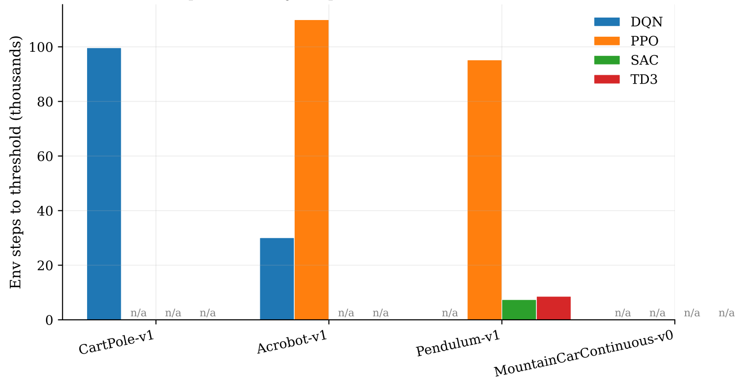
Sample efficiency: steps to reach the solved threshold
