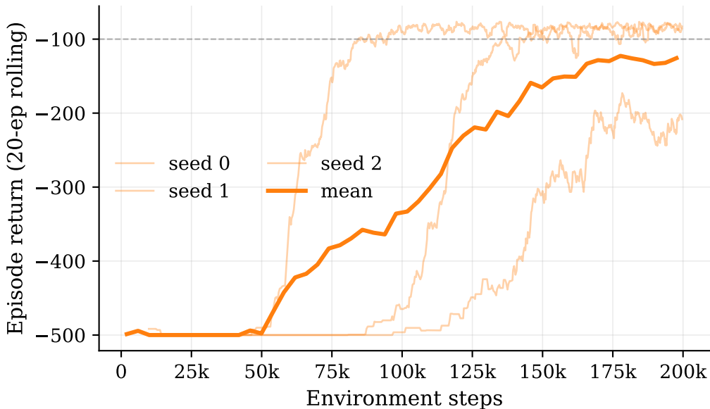
PPO on Acrobot-v1: per-seed curves
