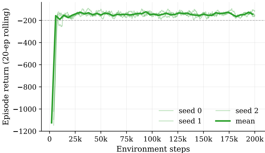
SAC on Pendulum-v1: per-seed curves
