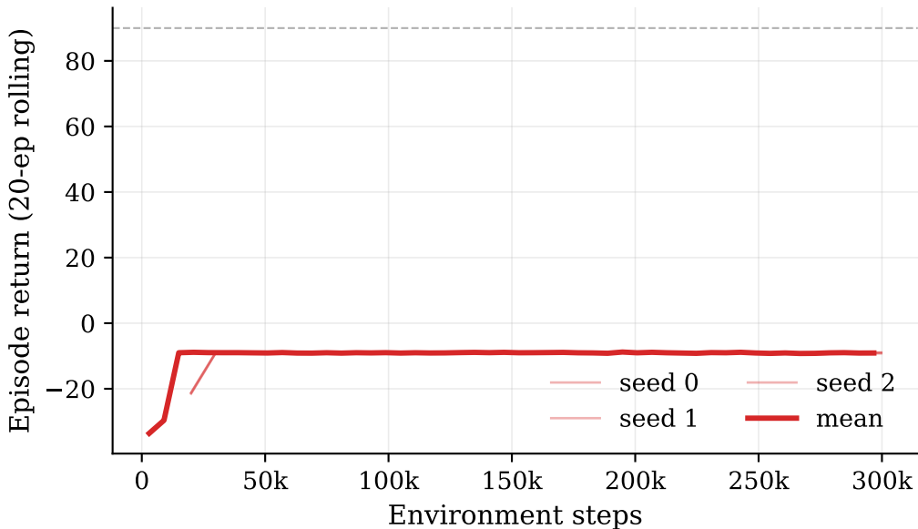
TD3 on MountainCarContinuous-v0: per-seed curves
