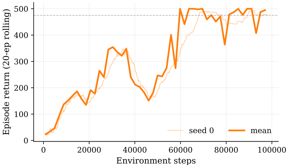
PPO on CartPole-v1: per-seed curves
