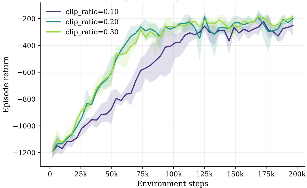
PPO clip ratio sweep on Pendulum-v1
