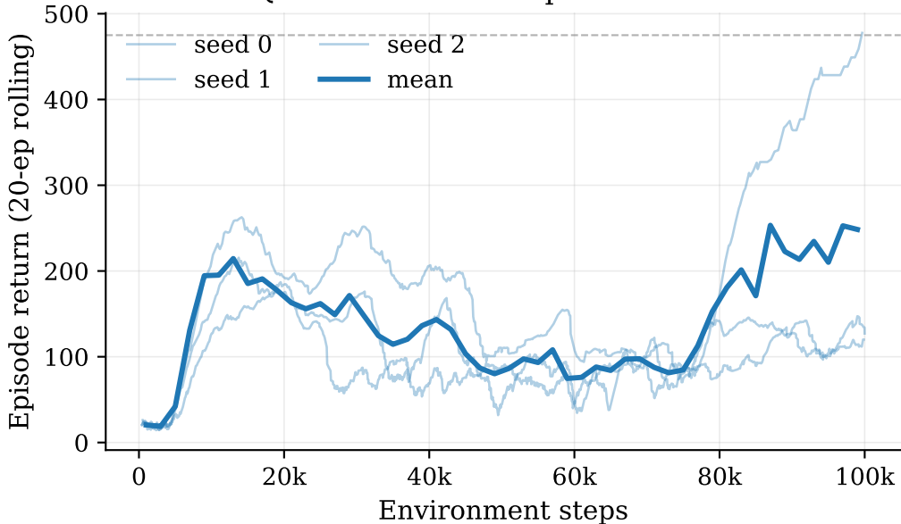
DQN on CartPole-v1: per-seed curves
