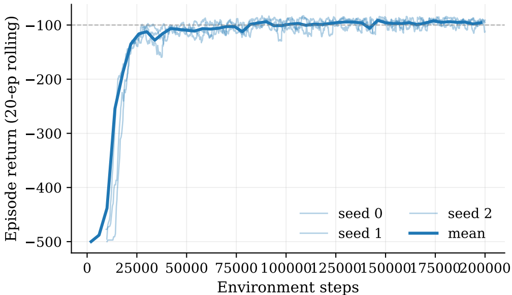
DQN on Acrobot-v1: per-seed curves
