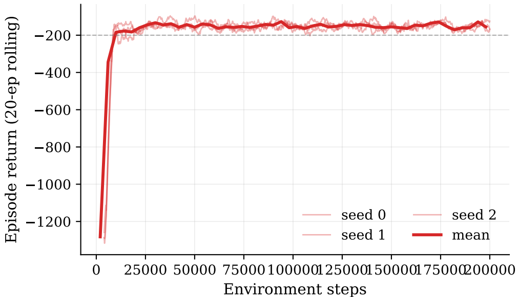
TD3 on Pendulum-v1: per-seed curves
