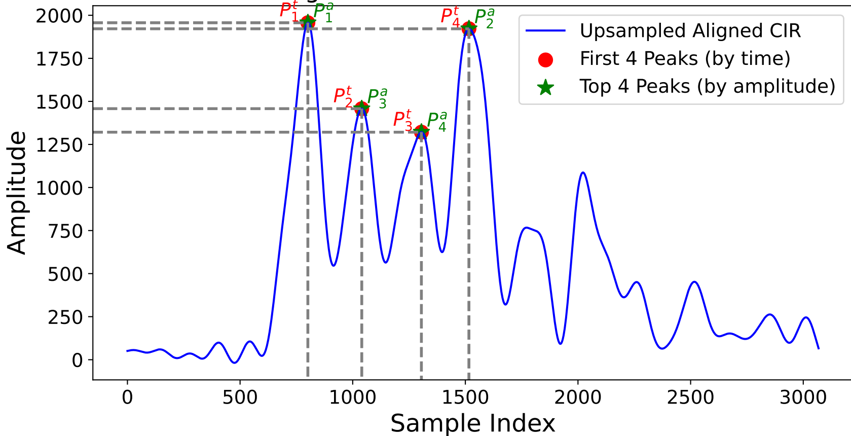
Aligned CIR with Detected Peaks
