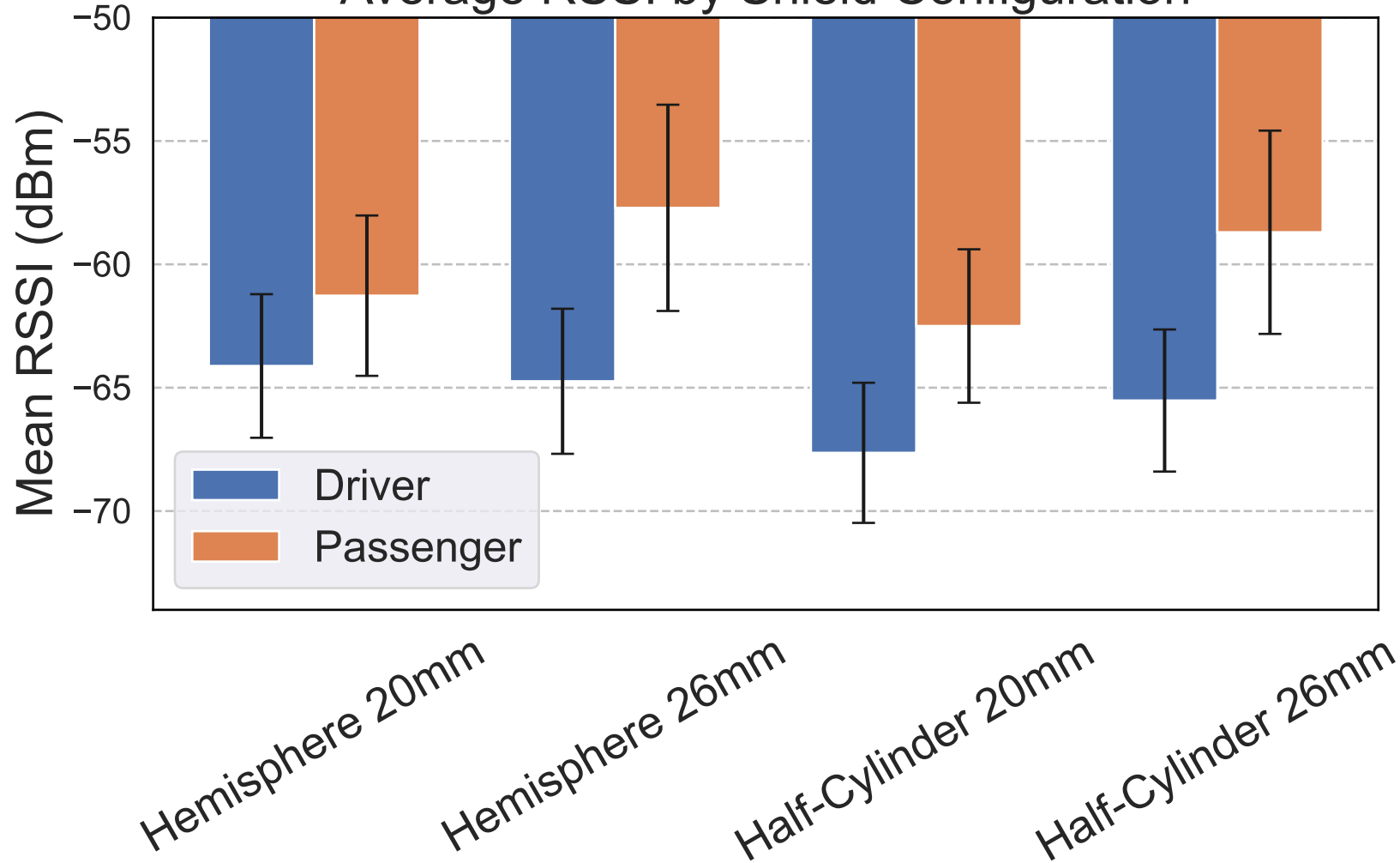
Average RSSI by Shield Configuration
