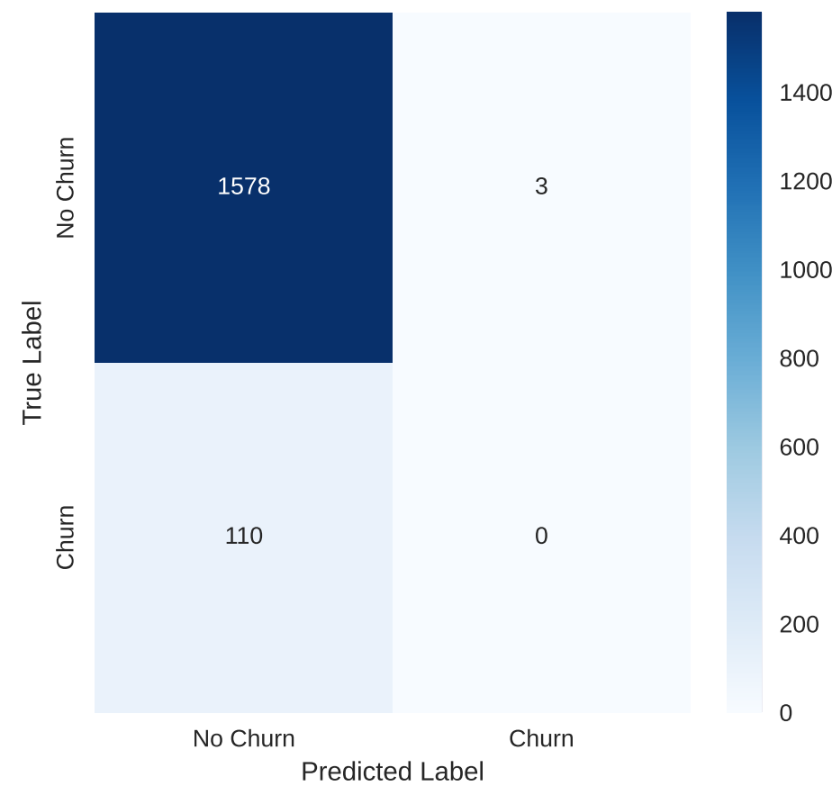
Naive Bayes
