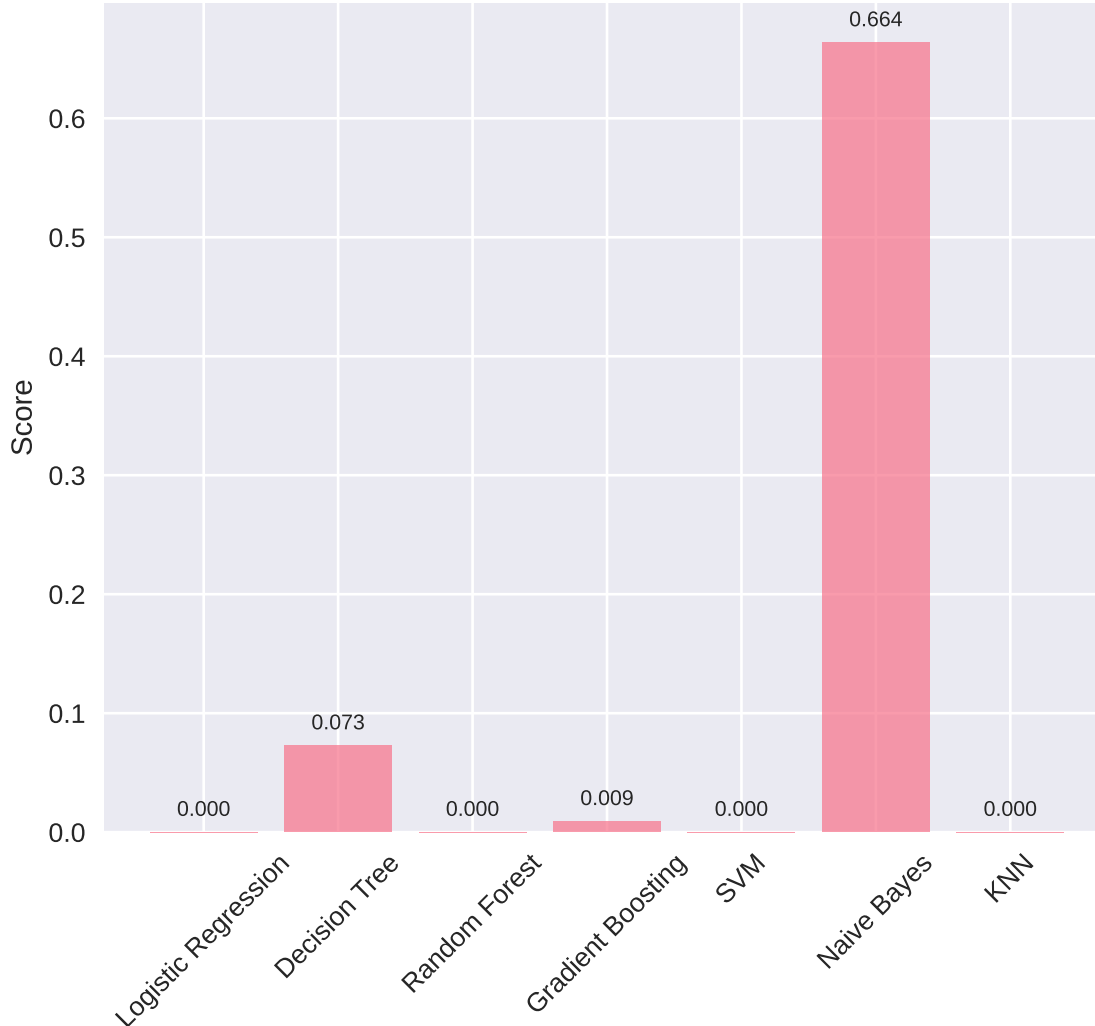
Recall
