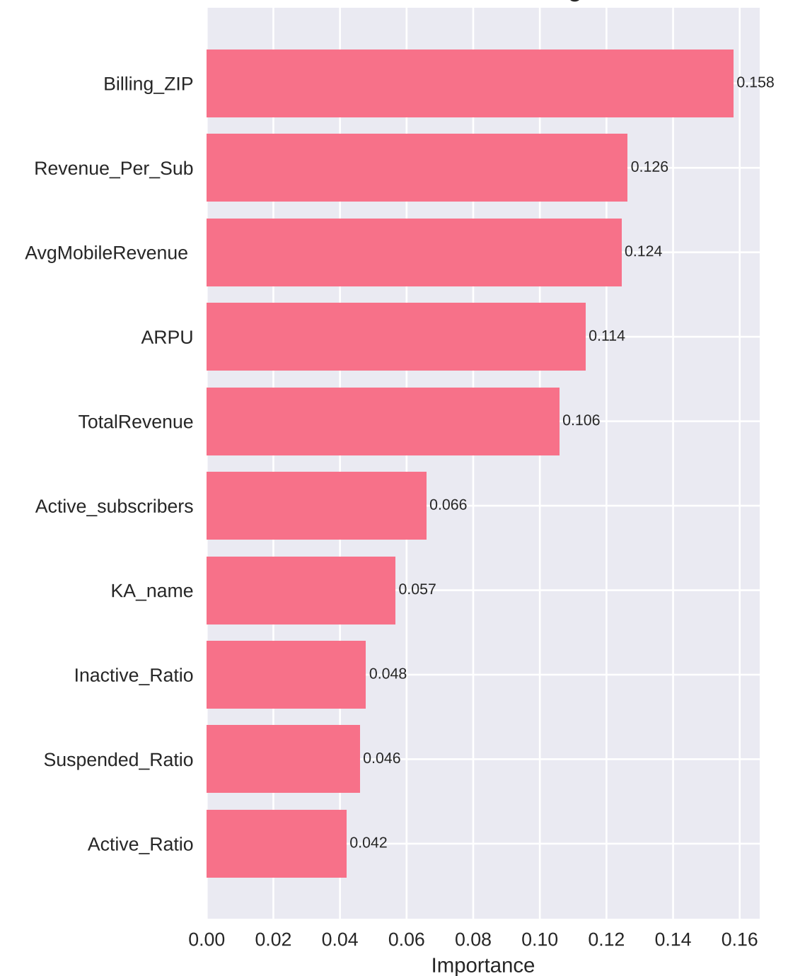
Gradient Boosting
