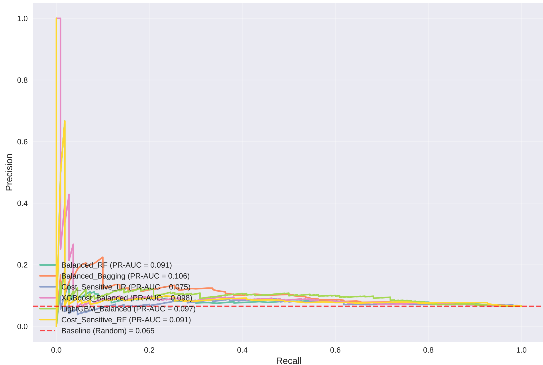
Precision-Recall Curves
