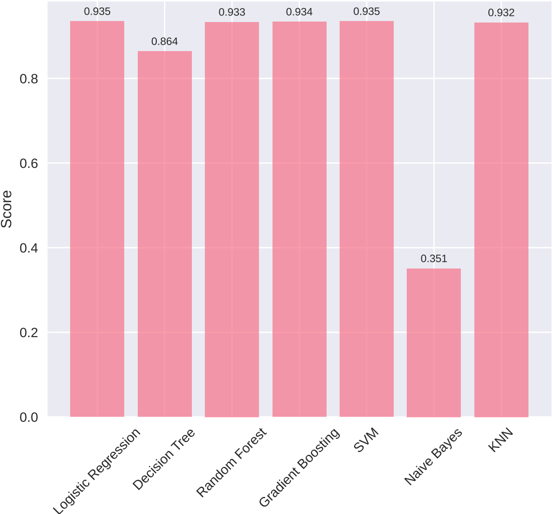
Accuracy
