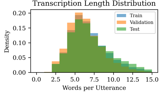
Fig. 10. Words per utterance across splits. Mean word count: 6.3 (train), 5.9 (validation), 6.5 (test). Range: 1–14 words. Mean word length: 5.60 characters.
