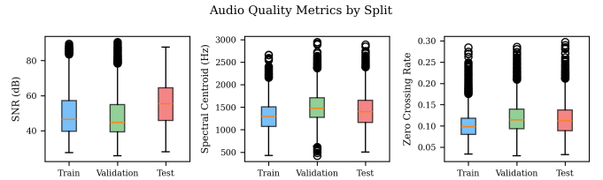
Fig. 7. Audio quality metrics by split. SNR values are consistently high (>25 dB), spectral centroids fall within the expected speech range (200–8000 Hz), and zero-crossing rates indicate clean recordings.
