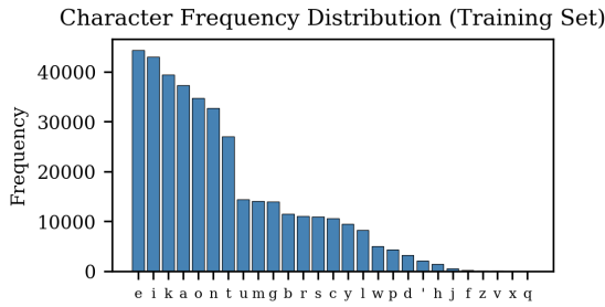
Fig. 3. Character frequency distribution in the training set. The distribution reflects Kalenjin’s phonological structure, with high-frequency vowels ( e , i , a , o ) and the consonant k .
