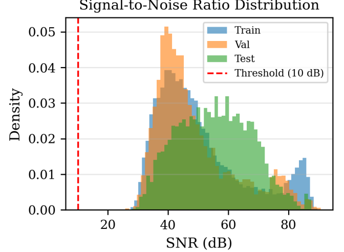
Fig. 13. SNR distribution with 10 dB minimum threshold (dashed red line). All retained samples comfortably exceed the threshold, with split means of 48.9–55.5 dB.
