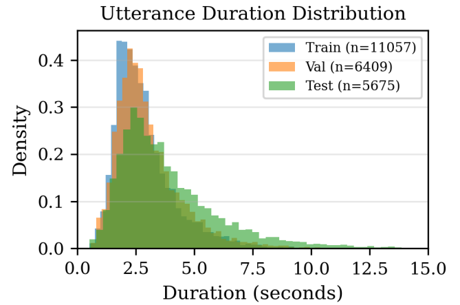
Fig. 10. Utterance duration distribution by split. The test split exhibits notably longer mean duration (3.89 s) compared to train (2.84 s), with a wider spread ( \sigma = 2.17 s vs. 1.30 s).
