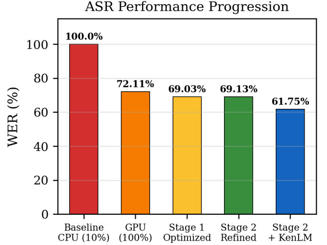
Fig. 14. WER progression across configurations. Data scaling (10%→100%) eliminated degenerate predictions; two-stage training and KenLM integration yielded cumulative 38.25 percentage point reduction.
