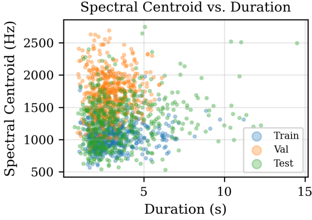
Fig. 11. Spectral centroid vs. utterance duration (500 samples per split). Shorter utterances tend toward higher spectral centroids, reflecting proportionally greater consonant energy.
