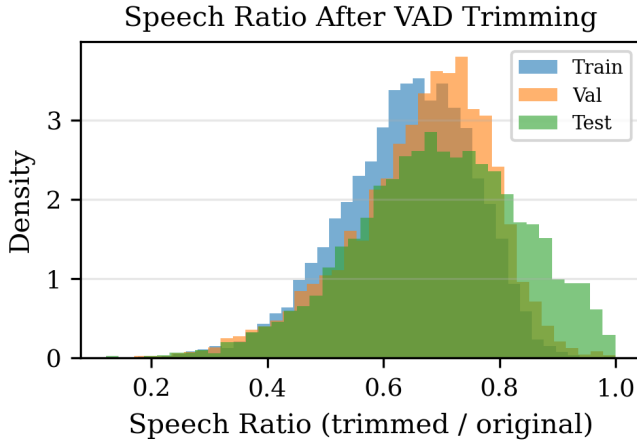
Fig. 6. Speech ratio distribution after VAD-based silence trimming. The majority of utterances retain 50–80% of their original duration, with the test split showing slightly higher speech ratios.
