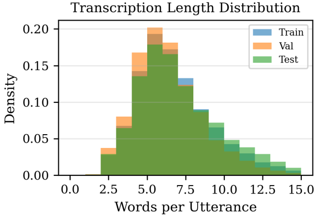
Fig. 12. Words per utterance across splits. Mean word count: 6.3 (train), 5.9 (validation), 6.5 (test). Range: 1–14 words. Mean word length: 5.60 characters.
