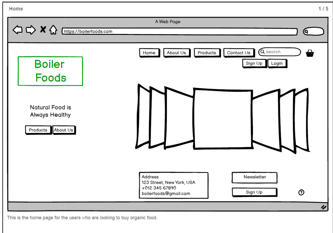
Figure1- Home page
