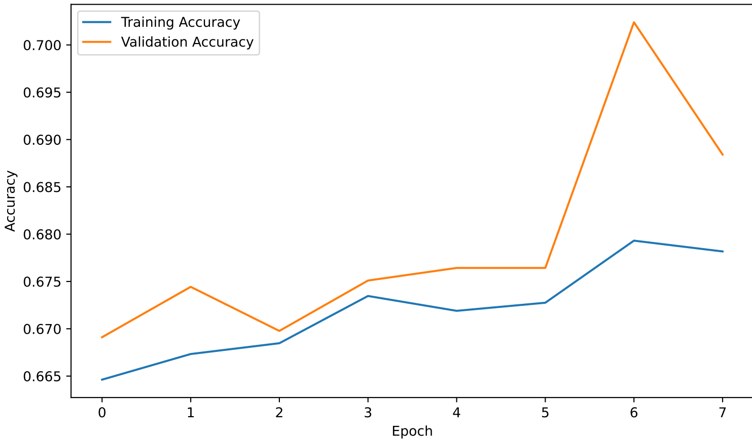
CNN Accuracy Curve
