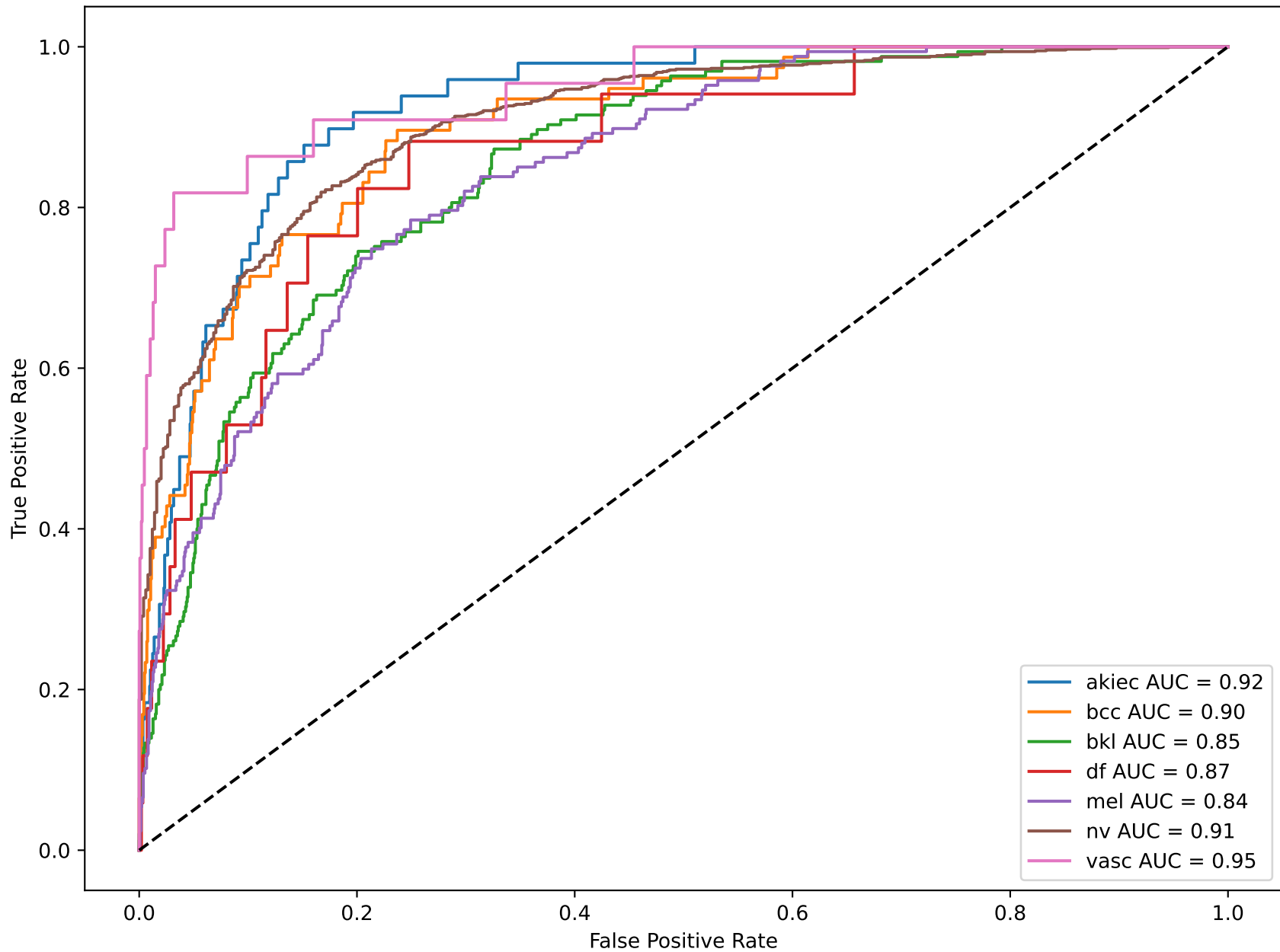
ROC Curve - MobileNetV2
