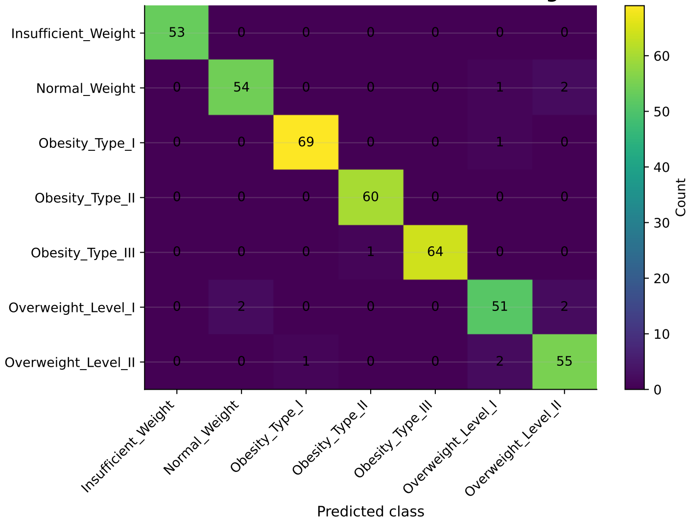
Confusion Matrix: Gradient Boosting
