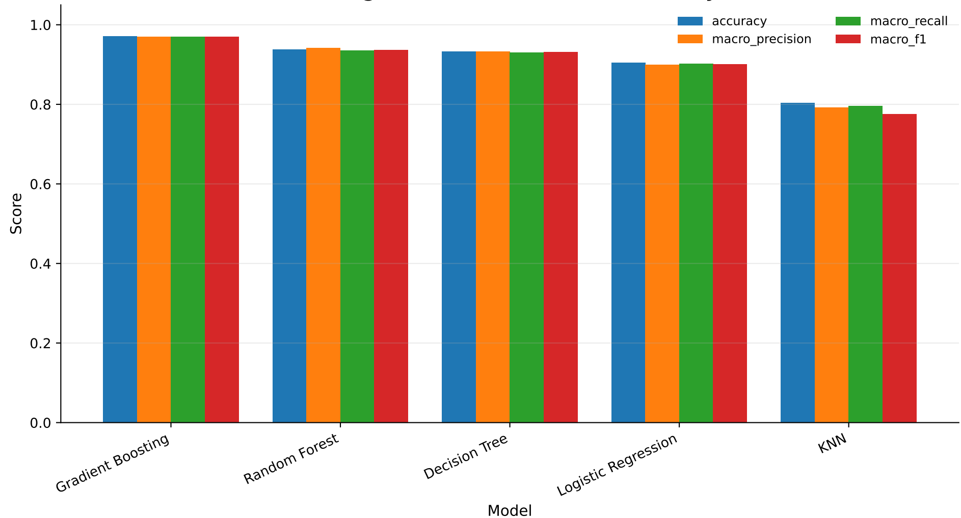
Machine Learning Model Performance for Obesity Prediction
