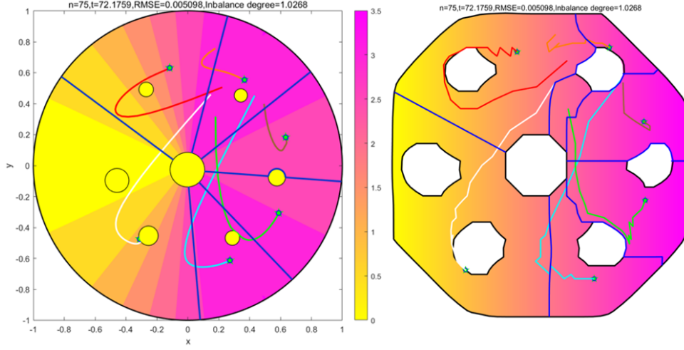
Figure 7: The coverage process and its indexes in the porous environment.
