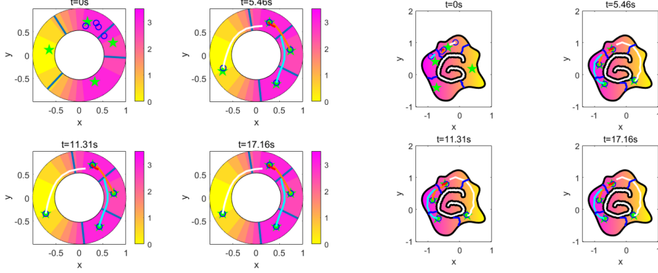
Figure 2: Coverage process on the mapped region \Xi and the original region (\Omega-O)\cup\partial O .
