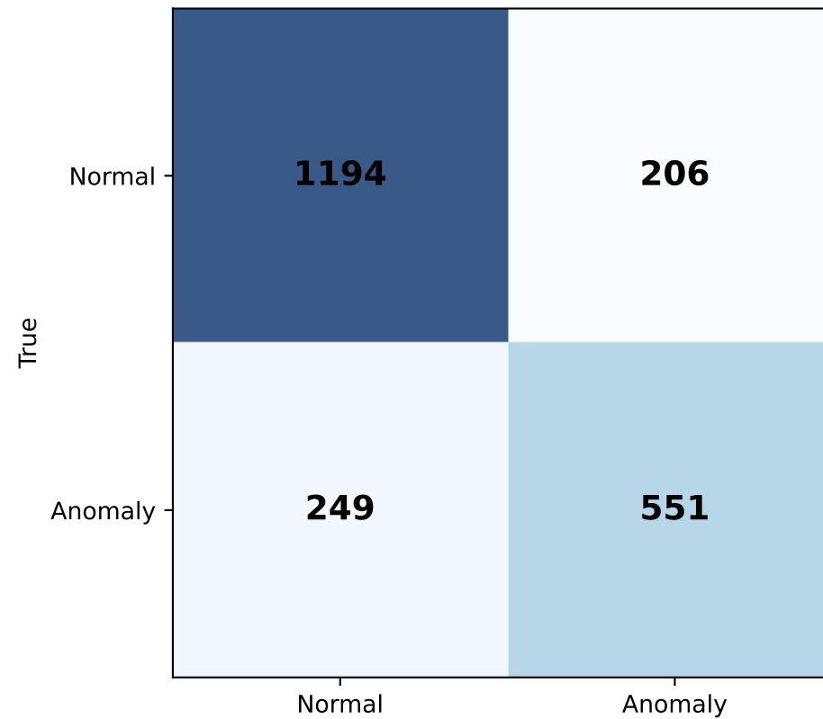
Image-Only Recall: 0.689
