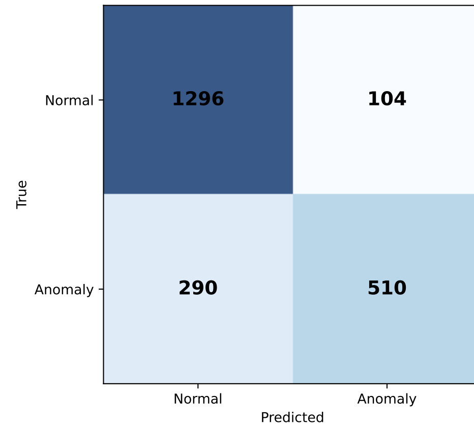
Lightweight Recall: 0.637
