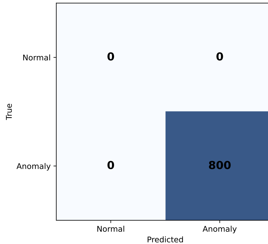
Dynamic-Only Recall: 1.000
