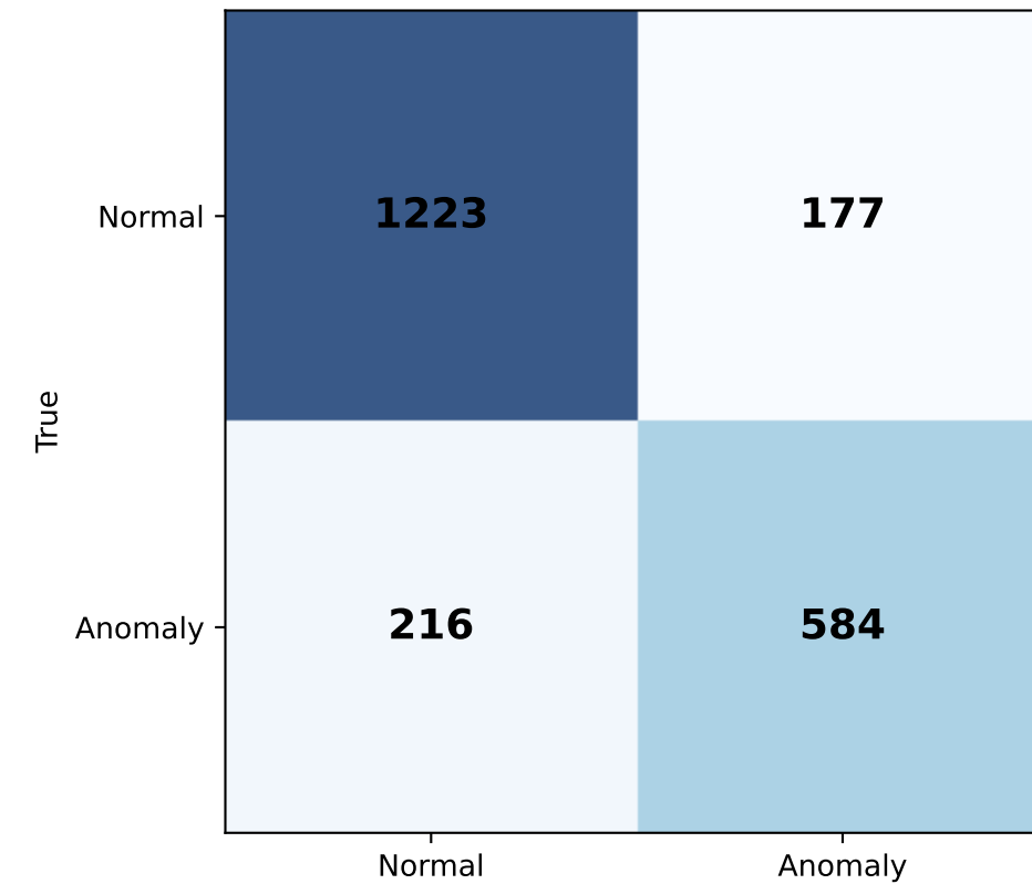
LiDAR-Only Recall: 0.730
