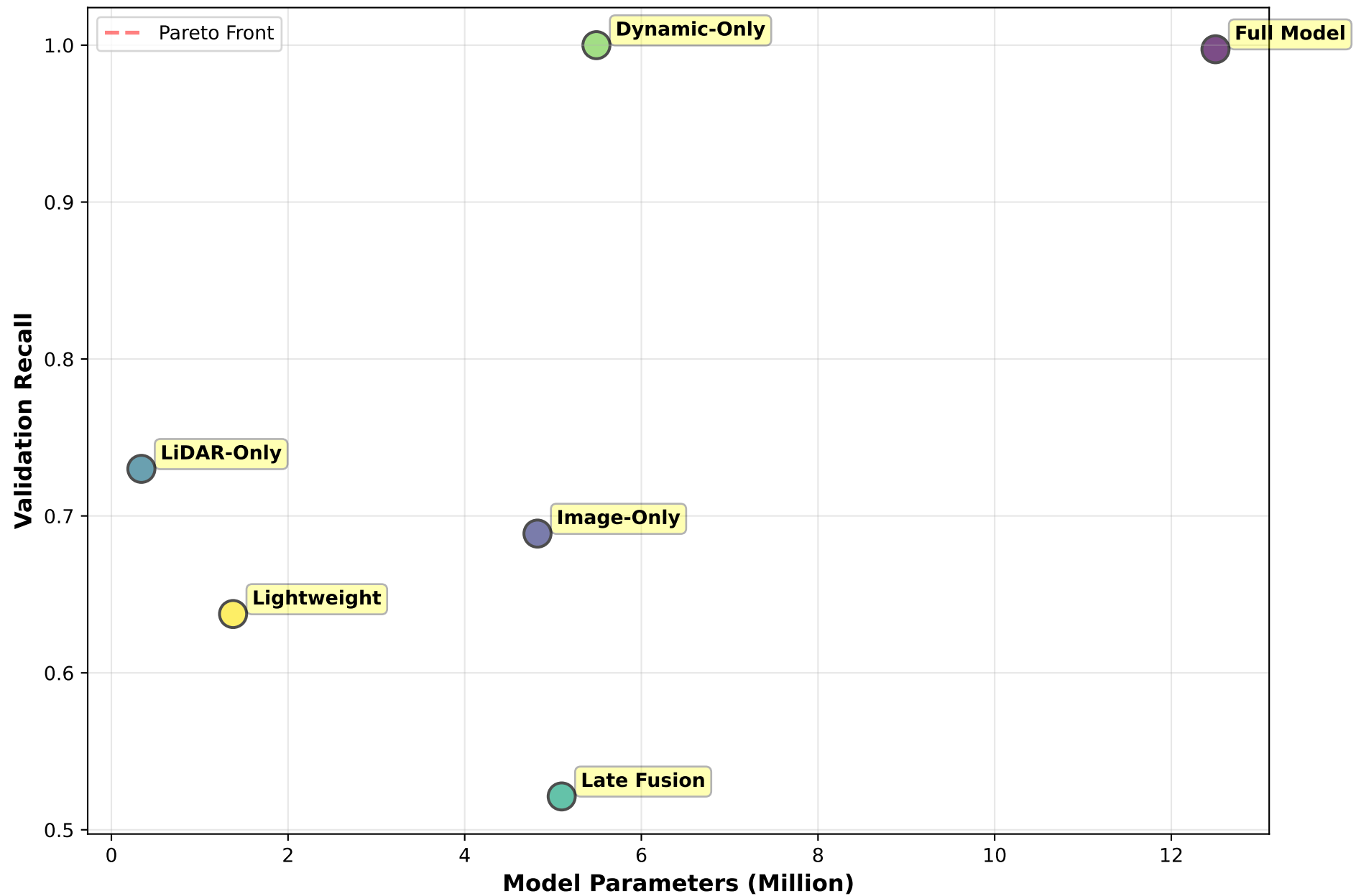
Parameter-Performance Trade-off
