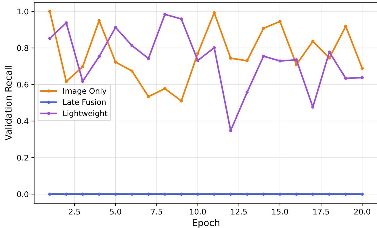
Recall Curves
