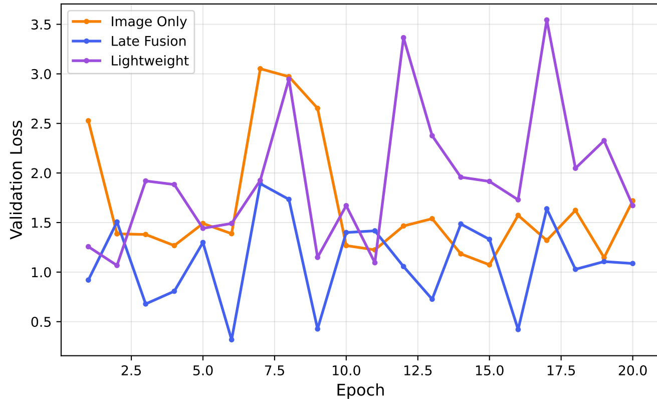
Loss Curves
