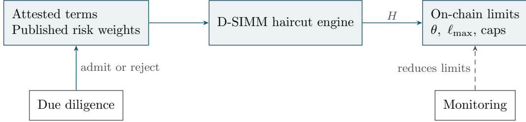
Figure 1: Attested terms and published risk weights feed the D-SIMM haircut engine. The haircut H sets the active on-chain limits with no iteration. Due diligence admits or rejects an asset, and monitoring can only reduce those limits.
