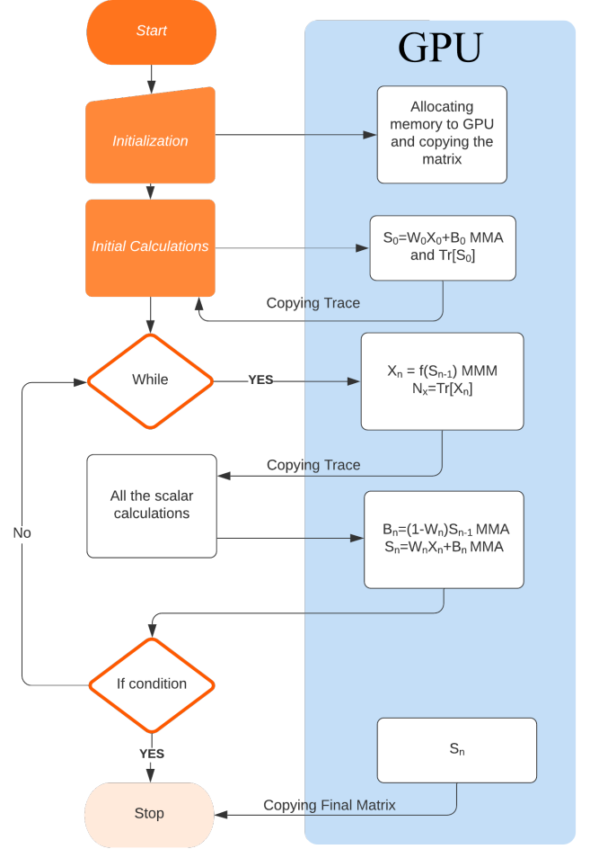
Fig. 2. Flow Chart of the implementation of the Deep NN Sp2 recursive Fermi-operator expansion, denoting the calling of different functions in the algorithm 1 and copying of data between CPU and GPU
