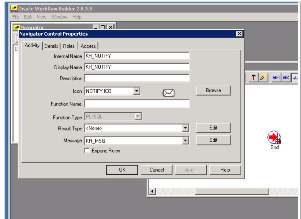
Final version: KH_NOTIFY with message KH_MSG.
