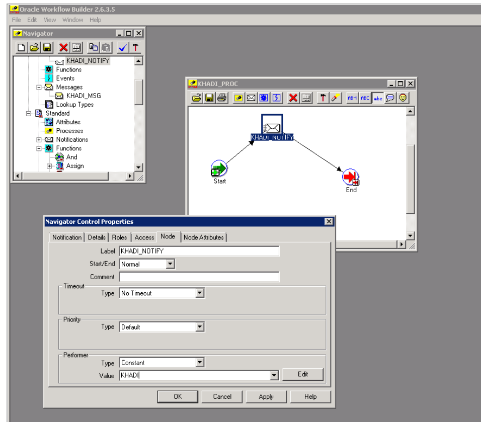
Process with Start > notification > End, and the Performer set on the Node tab.
