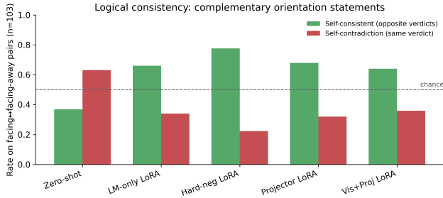
Figure 4. Self-consistency on complementary facing/facing-away relations across 7B conditions.
