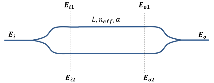
Fig. 3. Balanced MZI.
