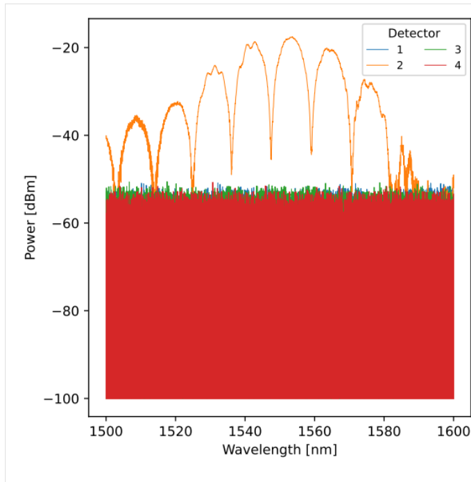
Fig. 16. Measured spectrum of MZI5 where \Delta L = 50\mu m (testing the fabrication/measurement variations)
