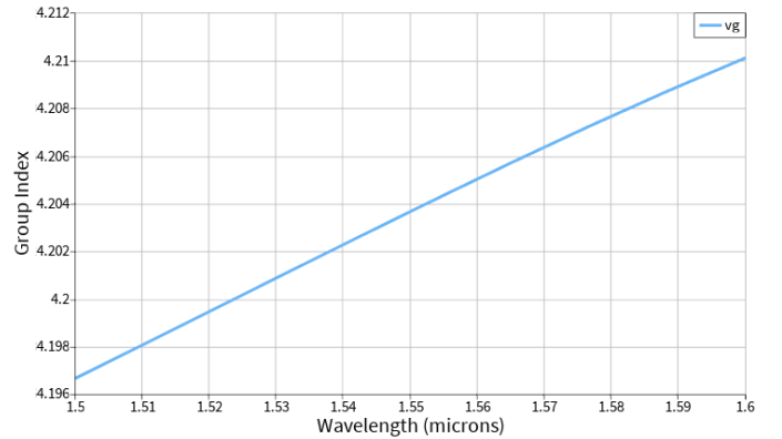
Fig. 8. Group index versus wavelength.
