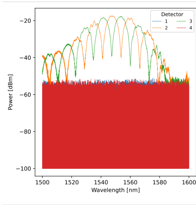
Fig. 17. Measured spectrum of MZI6
