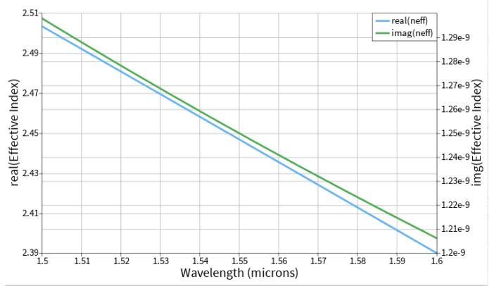
Fig. 7. Effective index versus wavelength.
