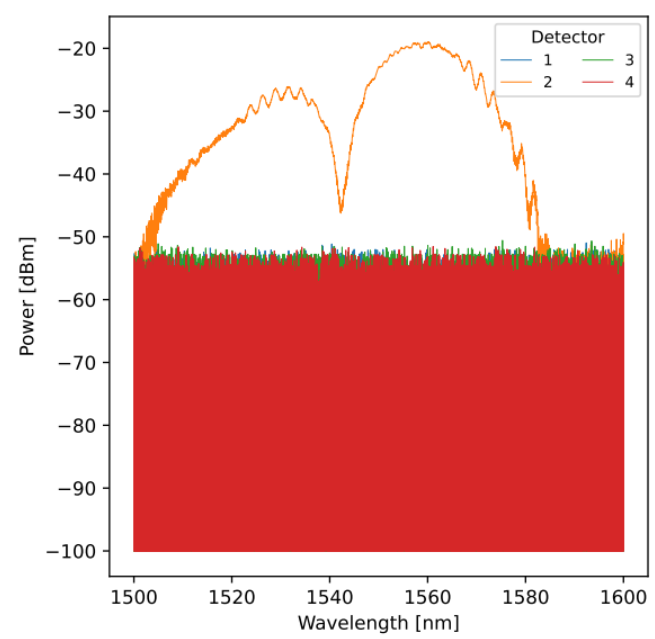
Fig. 15. Measured spectrum of MZI4 where \Delta L = 13\mu m
