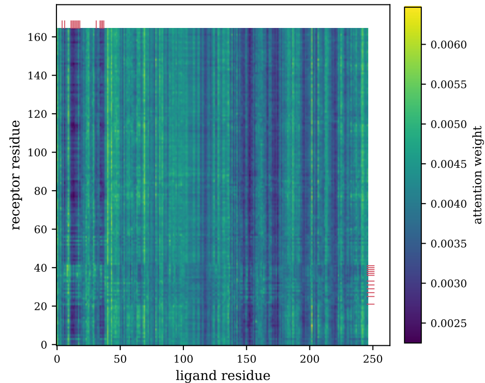
(a) cross-attention: receptor -> ligand
