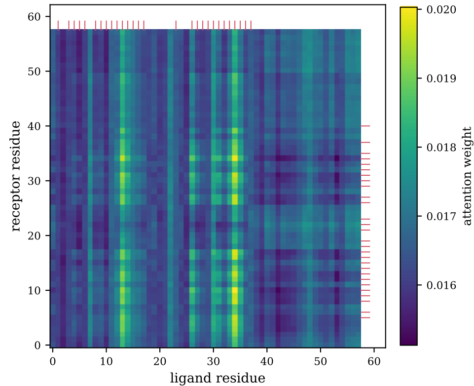
(a) cross-attention: receptor \rightarrow ligand
