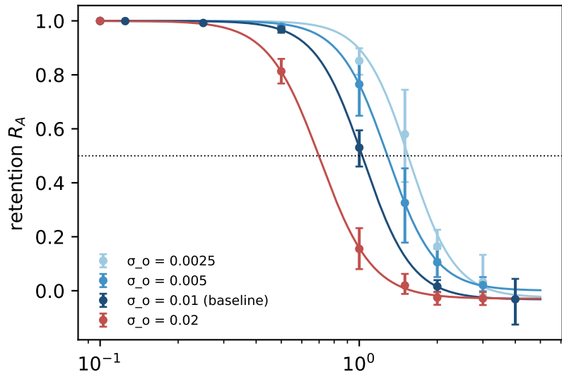
Sensitivity to the coupling-offset spread \sigma_o
