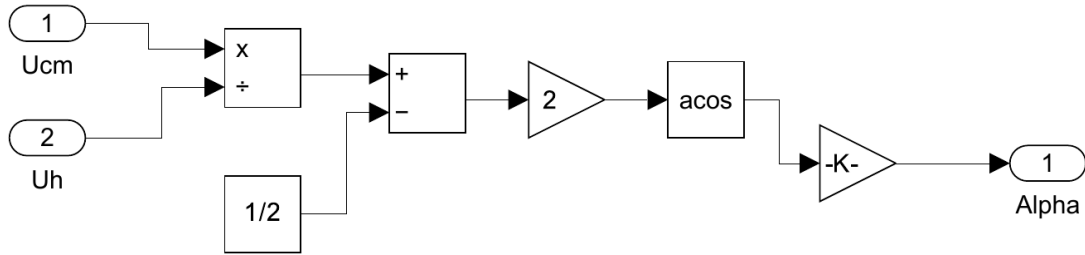
Figure 1. The firing-angle generator subsystem. It computes \alpha = \arccos(2U_{cm}/U_h - 1) , the inverse-cosine law that linearises the thyristor bridge.
