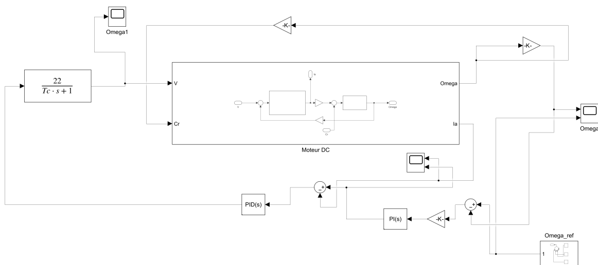
Figure 7. Transfer-function cascade block diagram: the idealised design model, matching Sections 2 to 4 one-to-one.
