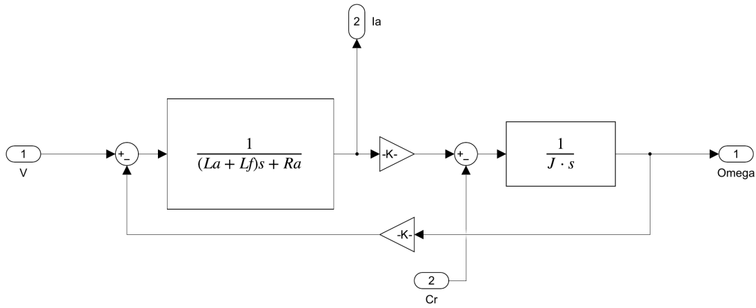
Figure 2. The DC machine subsystem: the armature admittance 1/((L_a + L_f)s + R_a) produces the current, k\Phi converts it to torque, 1/(Js) integrates to speed, and k\Phi\omega is fed back as the back-EMF.
