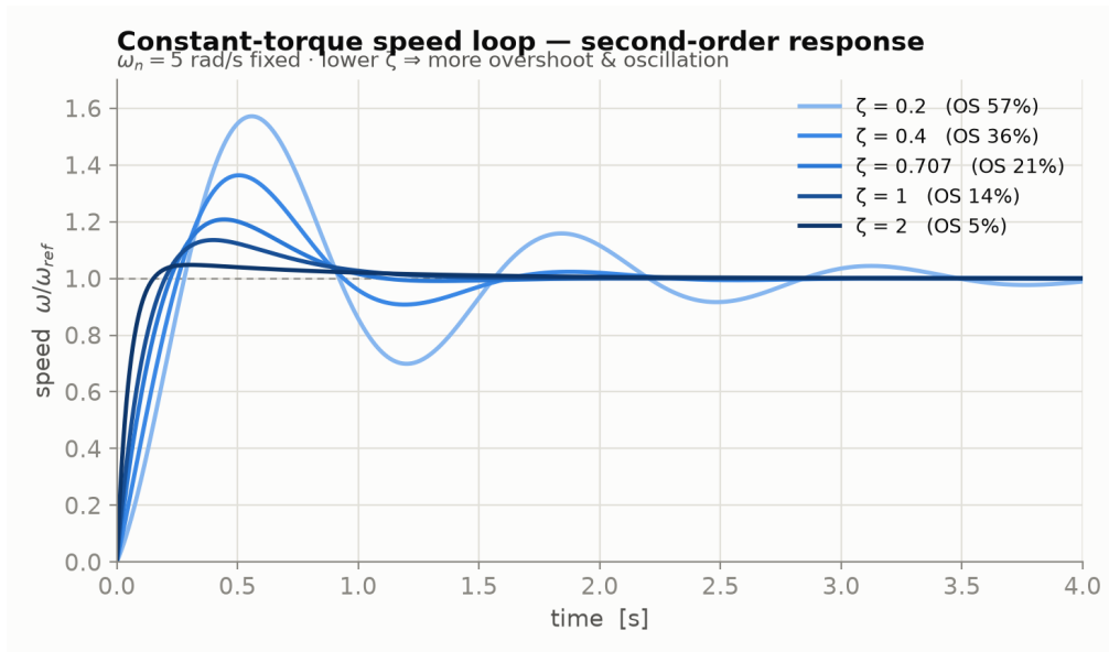
Figure 5. Second-order speed loop: the damping ratio sets the overshoot and the oscillation, at fixed \omega_n = 5 \text{ rad/s} .
