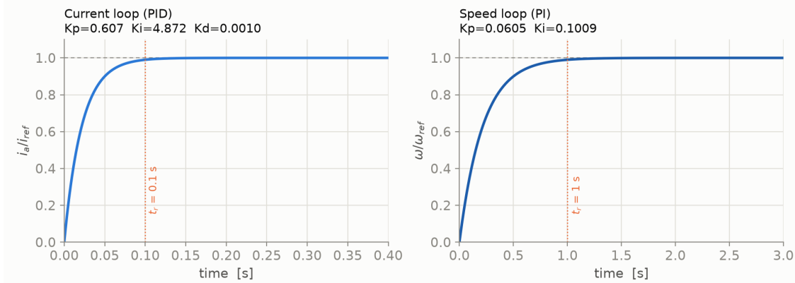
Figure 3. Step responses at the designed operating point: inner current loop (left) and outer speed loop (right), showing the deliberate ten-to-one time-scale separation.
