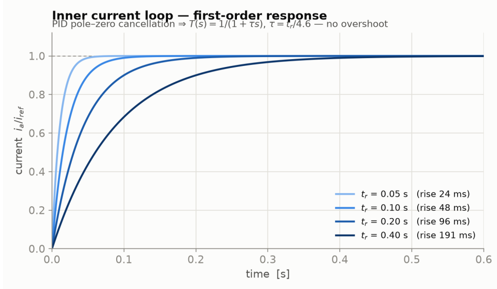
Figure 4. First-order current loop: the response-time target sets the rise time, with no overshoot at any setting.
