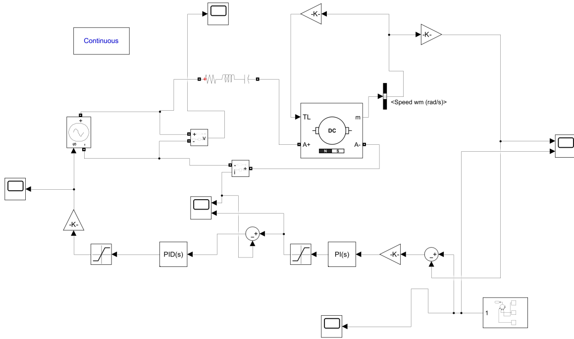
Figure 8. Intermediate physical model: the genuine Simscape DC Machine block driven by an averaged controlled voltage source.
