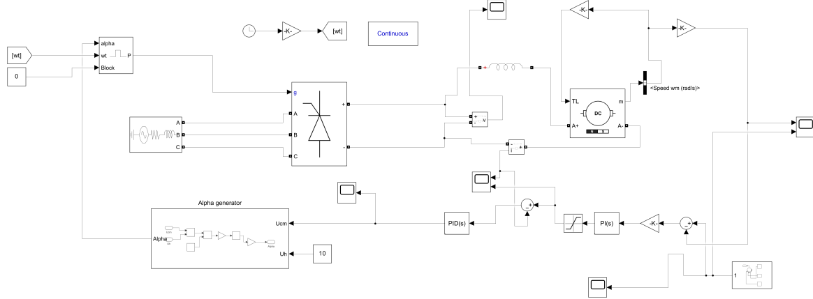
Figure 9. Full physical model: three-phase source, six-pulse thyristor bridge, firing-angle generator and synchronised pulse generator, smoothing inductor and DC machine.
