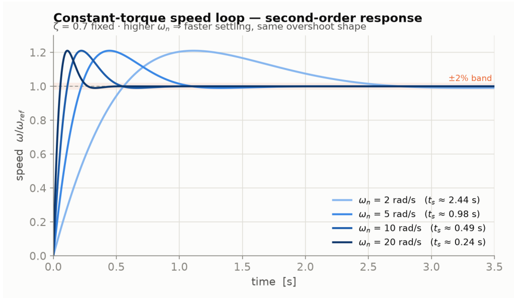
Figure 6. Second-order speed loop: the natural frequency sets the settling time, at fixed \zeta = 0.7 .
