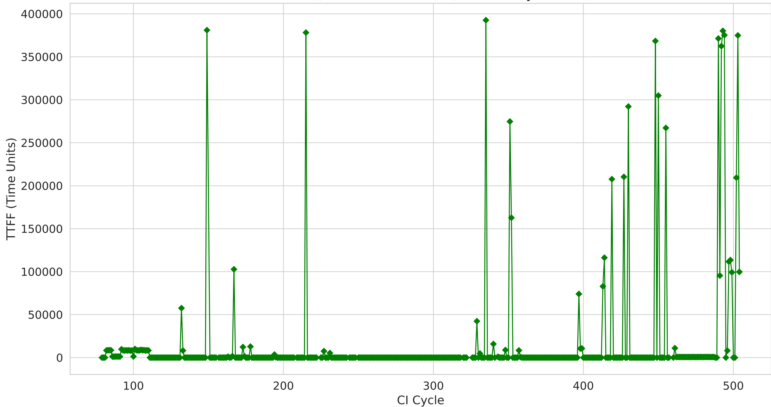
TTFF (Time to First Failure) Over CI Cycles
