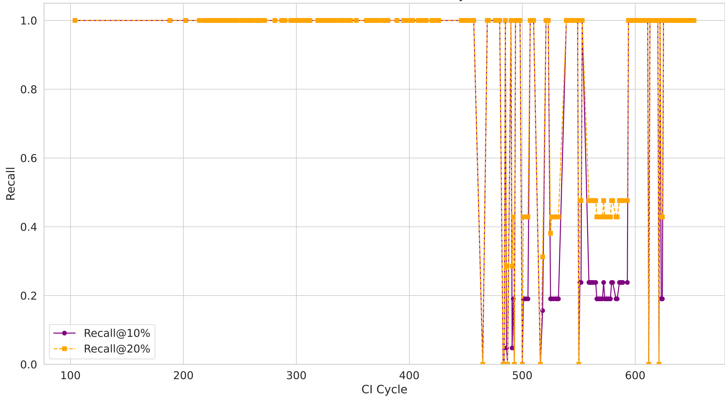
Recall Fluctuation Over CI Cycles
