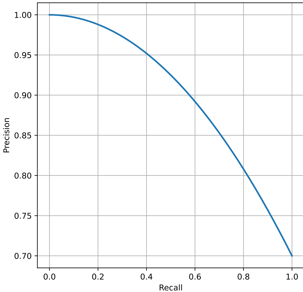
Precision-Recall Curve
