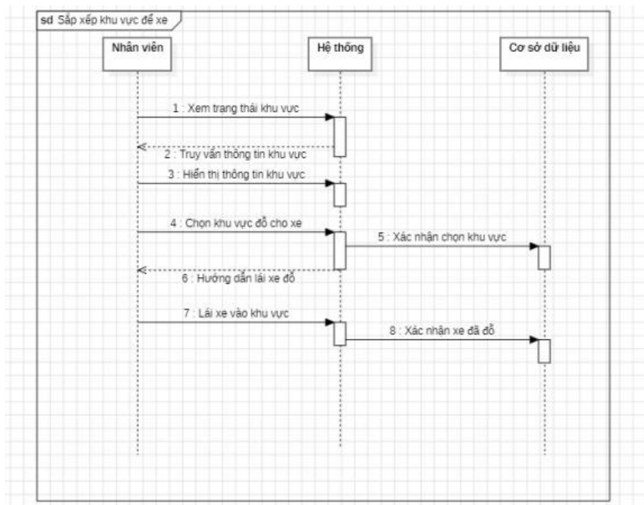
Sequence diagram
